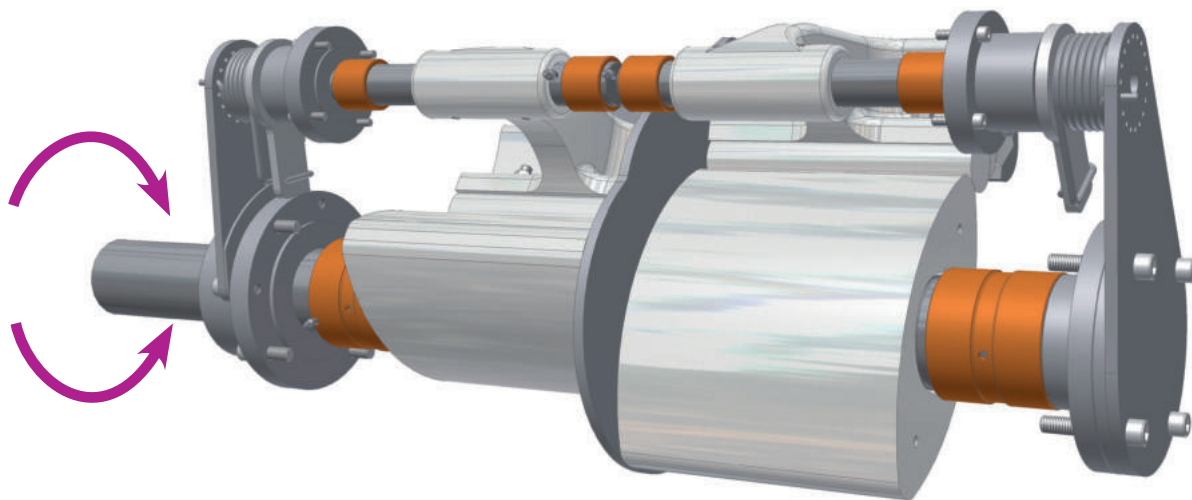
90° twin piston configuration
