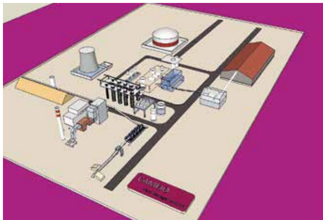
CAMEIO™ Plant Manager Solution - Simulation of all the lines of the sugar cane factory, power house, distillery, utilities and calculation of the revenues.
